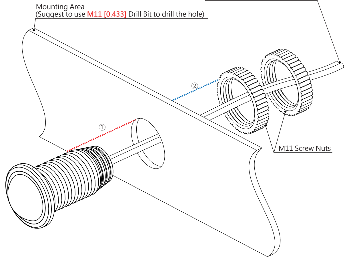
INSTALLATION DIAGRAM
