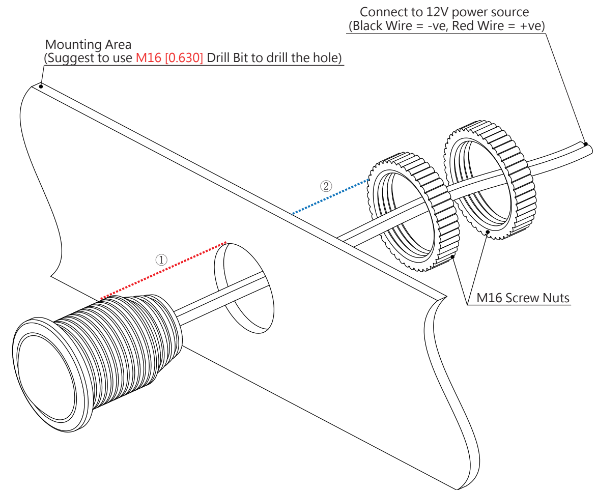
INSTALLATION DIAGRAM
