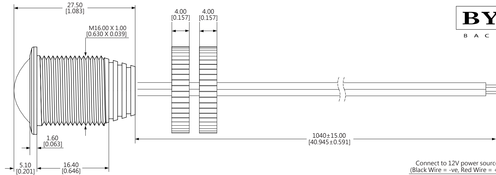
SIDE VIEW
